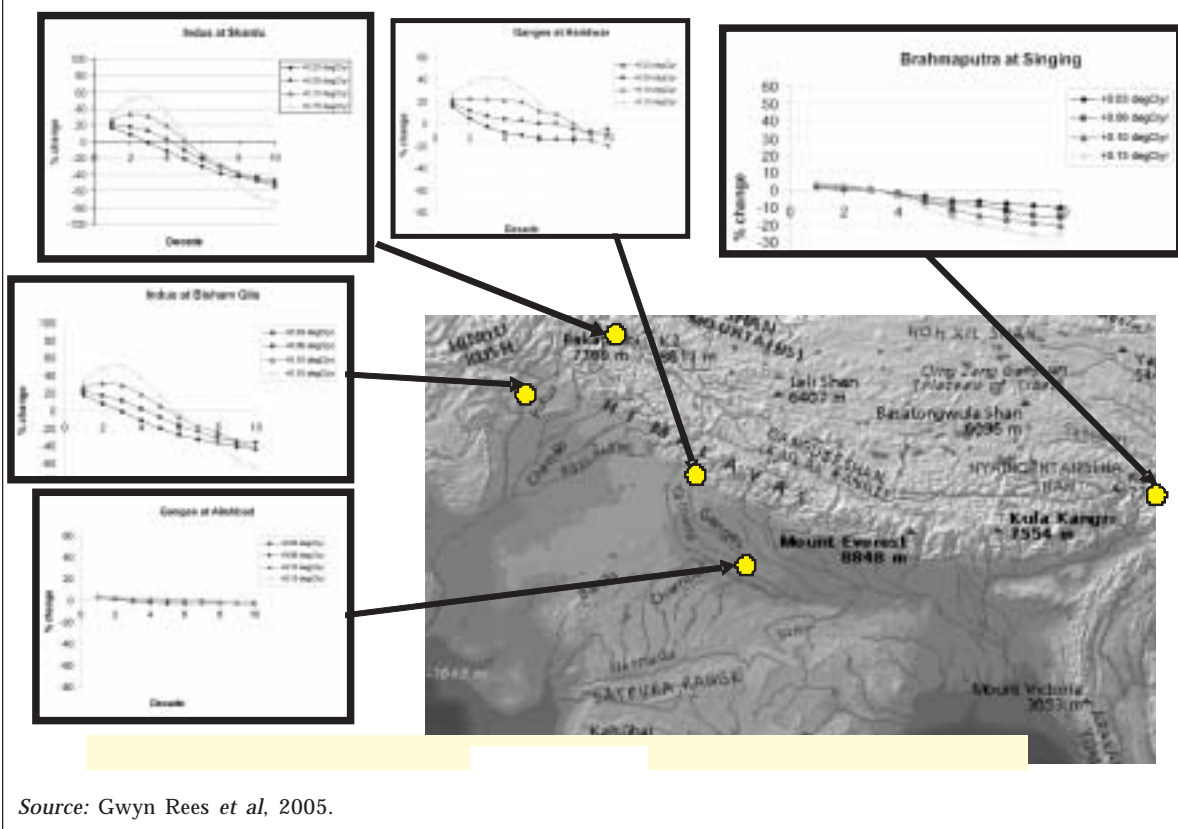
Figure 2.7: Simulated effects of deglaciation on Himalayan river flows over 10 decades
