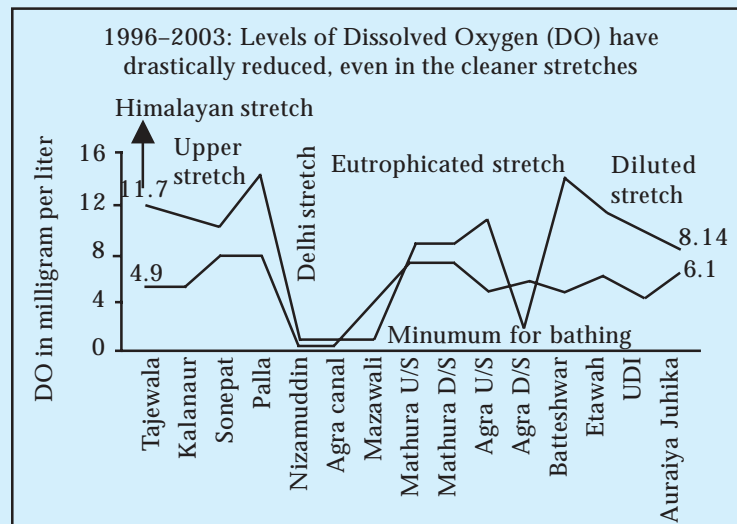
Figure B2.1: Yamuna River dissolved oxygen
