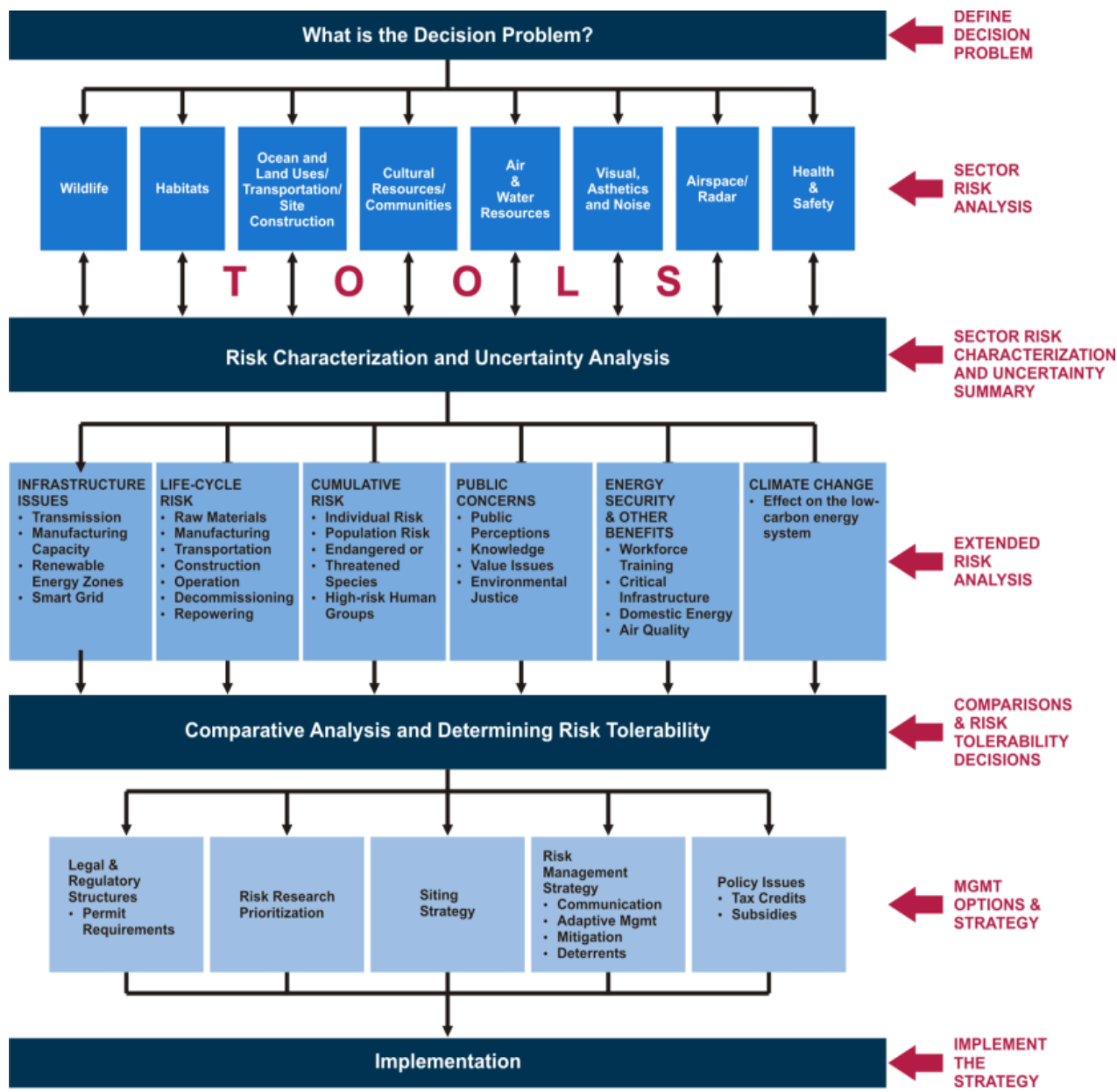
Figure 8-2. A framework for integrated risk analysis of gigawatt-scale wind energy deployments
